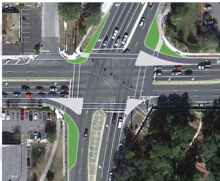
Figure 2 - SR 26 and Waldo Road, Compact Design
